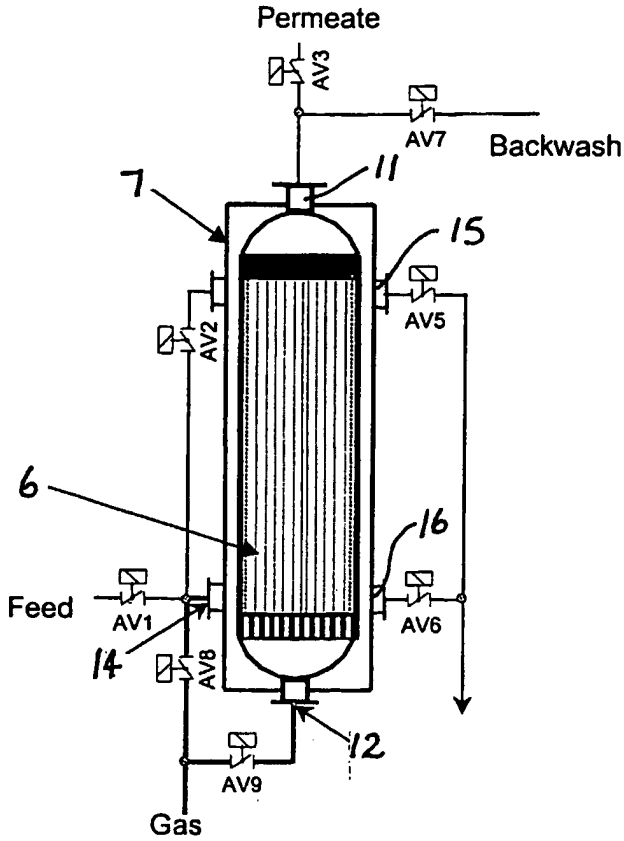
Figure 5 Alternative Air Injection
